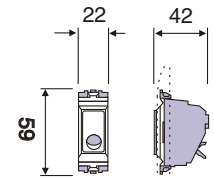
Cord unit
