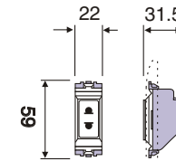
Universal Socket unit
