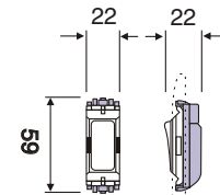
All switch and indicator modules
